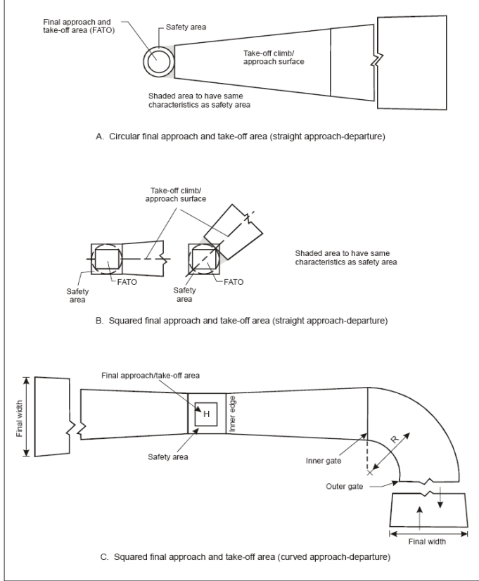
Figure 4-4. Take-off climb/approach surface (non-instrument FATO)
