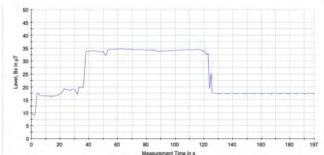
Braking-SP2ADC@70cm-Bx_M46
