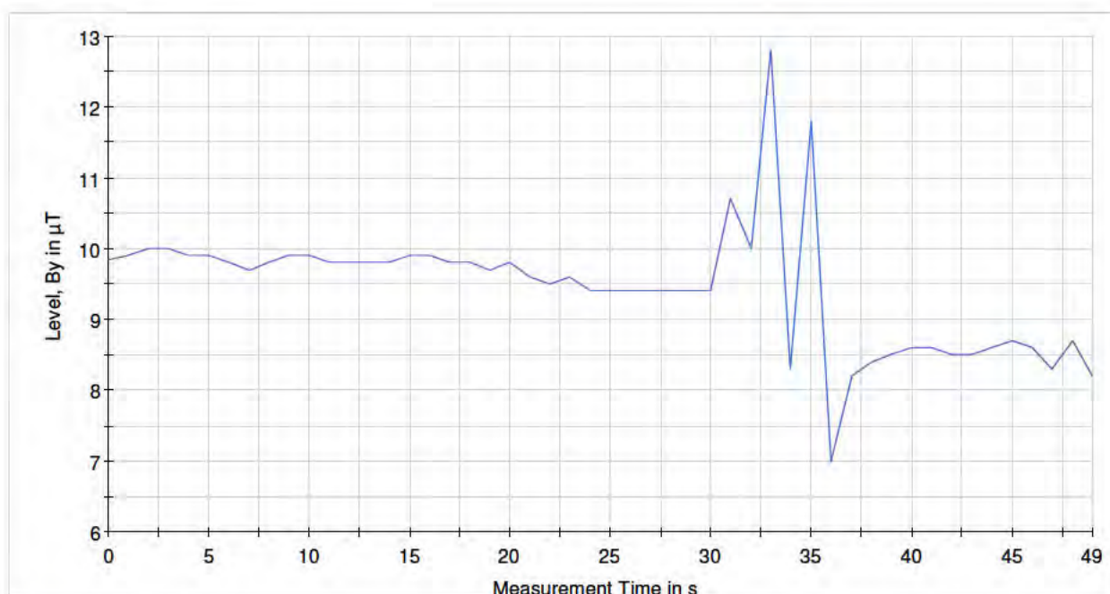
— Transit@30cm-By_M71
