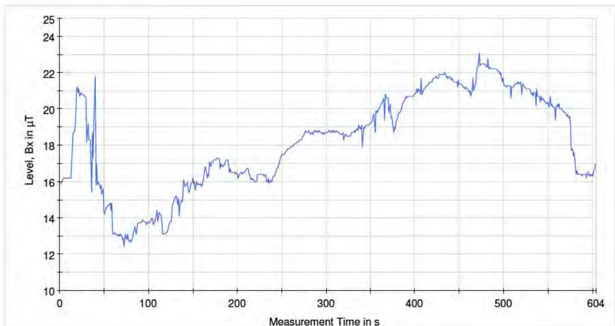
— Transit@1m-Bx_M108
