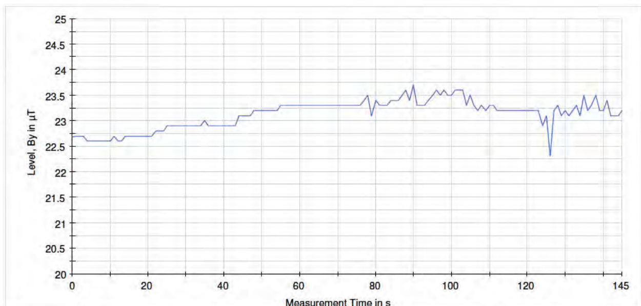
Braking-SP2ADC@1m-By_M112
