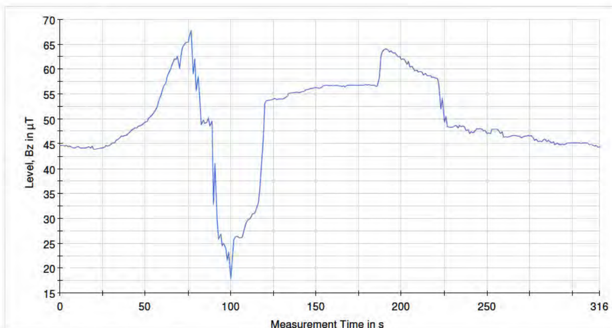
Accel@1m-Bz_M59
