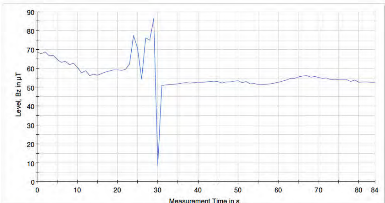
Transit@70cm-Bz_M52
