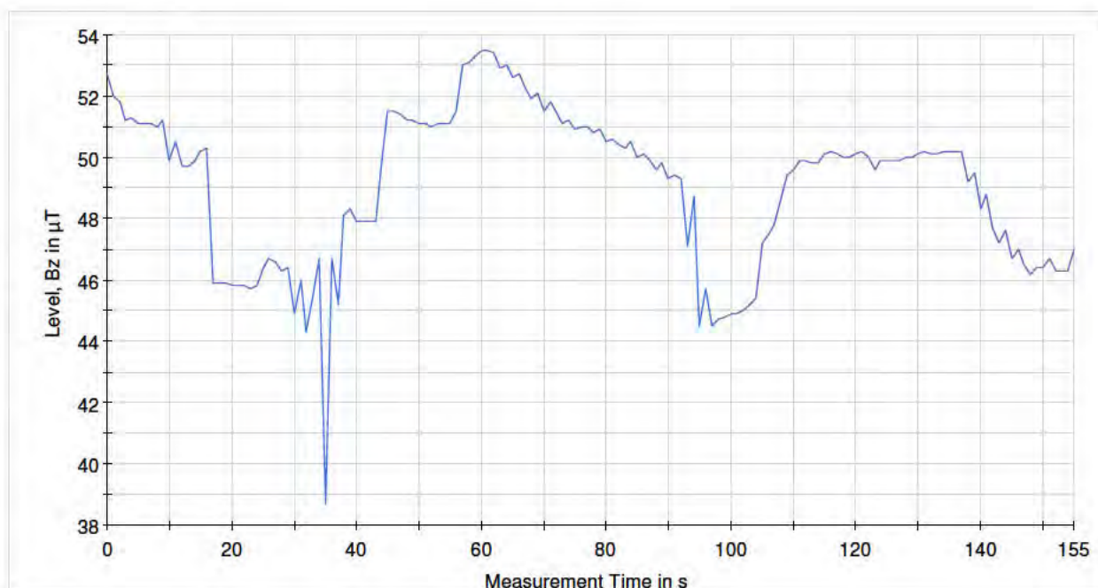
— Transit@1m-Bz_M55
