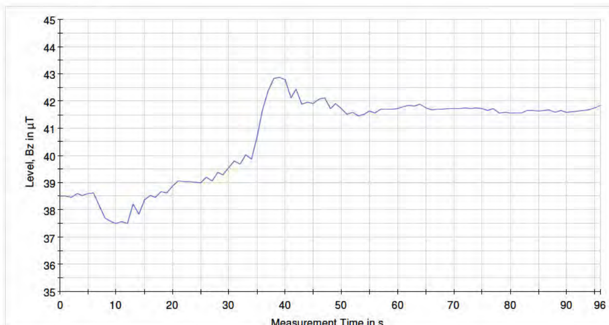
— Transit@1m-Bz_M130
