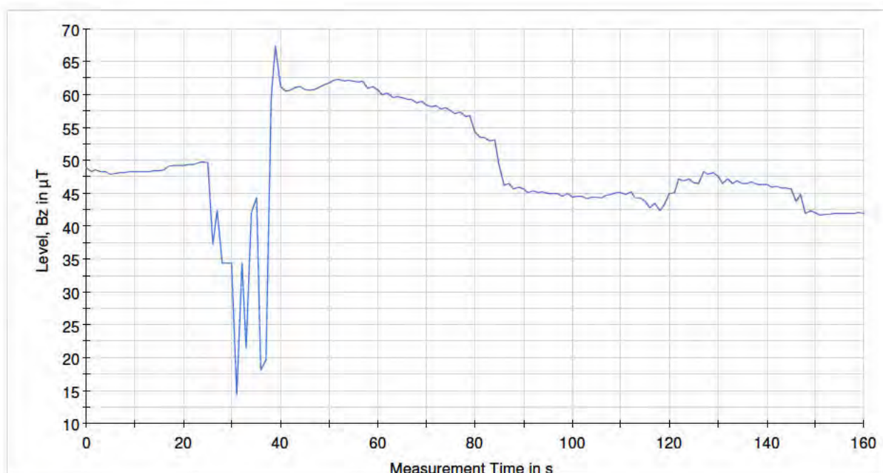
— Transit@1m-Bz_M37
